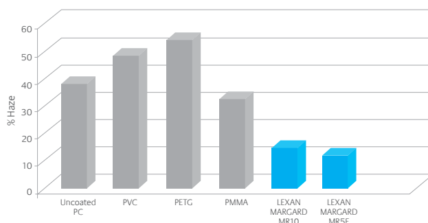
FIGURE 3 TABER ABRASION ASTM D1044 test at 500 cycles
